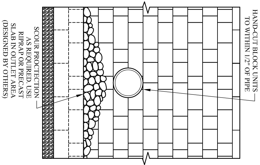
ELEVATION VIEW
