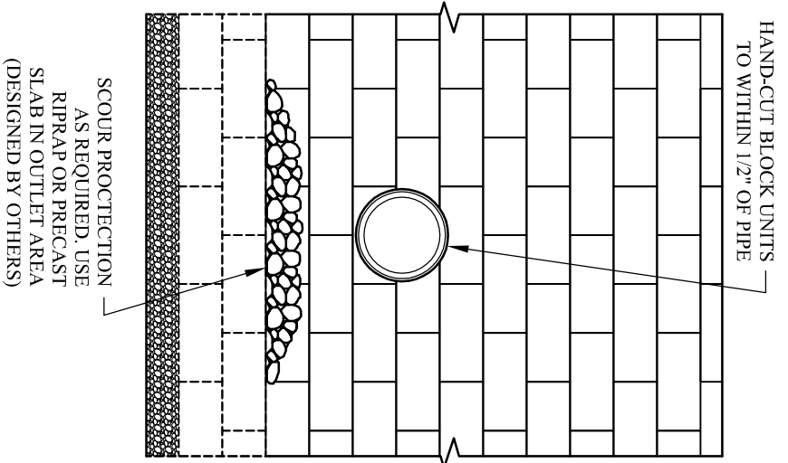
ELEVATION VIEW
