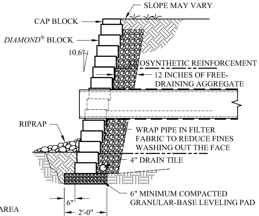
SECTION VIEW
