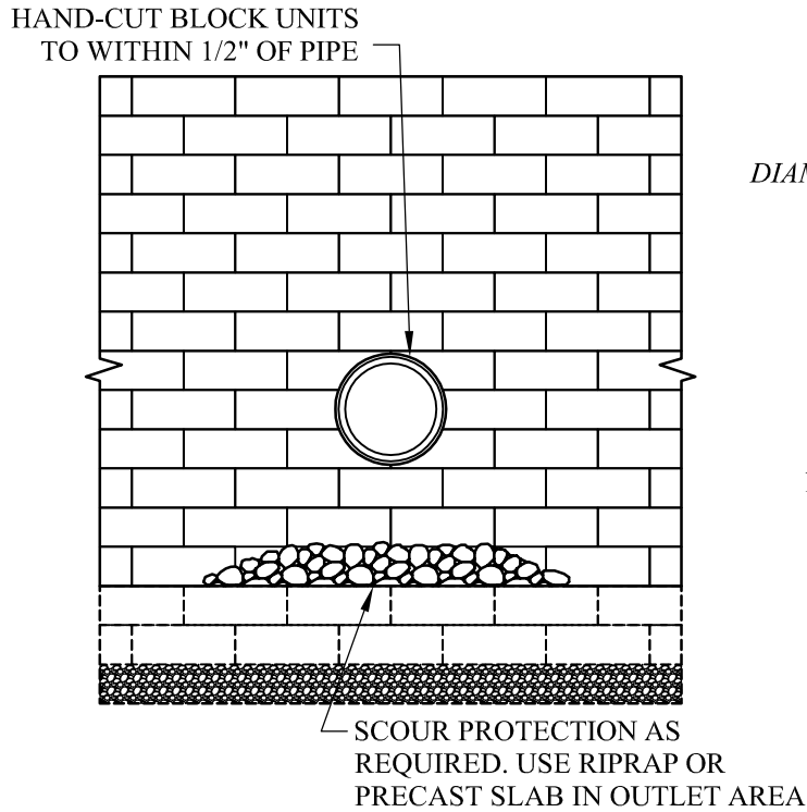
ELEVATION VIEW
