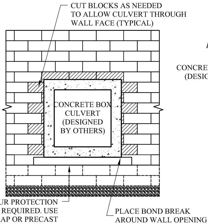
ELEVATION VIEW
