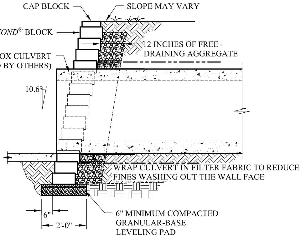
SECTION VIEW
